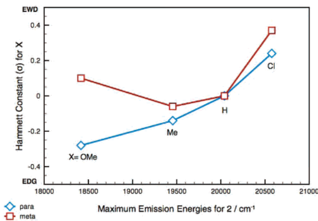
Figure 10. Correlation between \sigma_p and \sigma_m Hammett constants 41 versus emission energy for 2a–2d in 1.0 \times 10^{-5} M DMSO solution.
